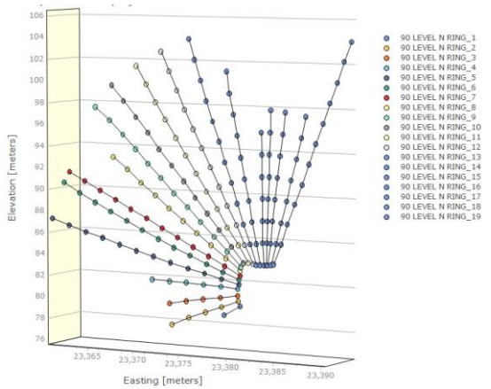
Blast ring section 3D-view
